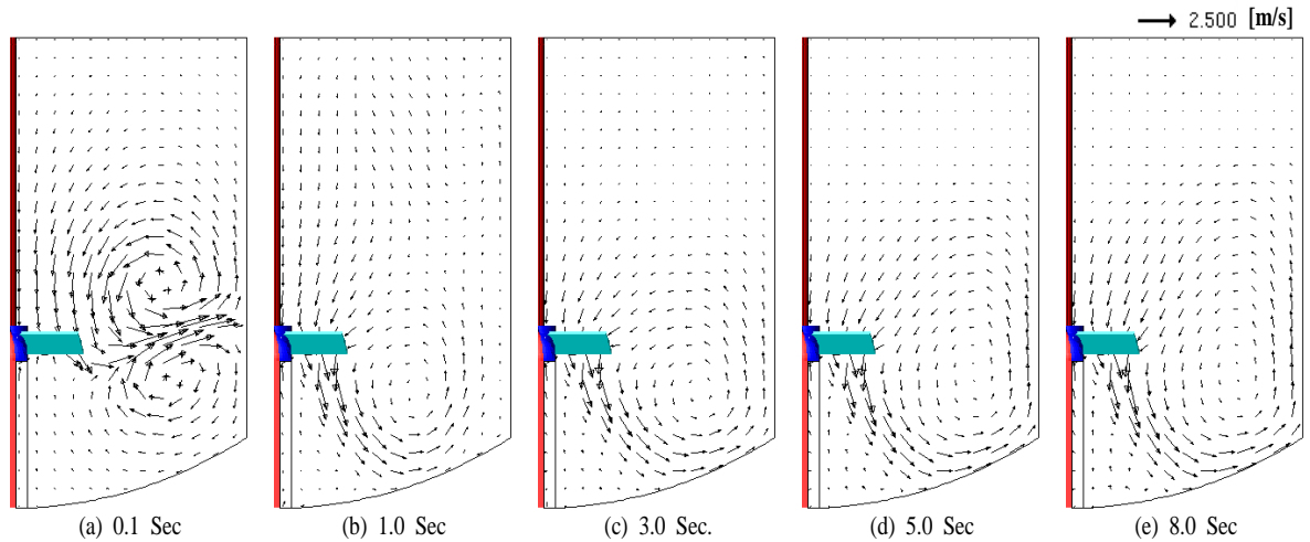
Fig. 4 Plot section of velocity vector of liquid phase
