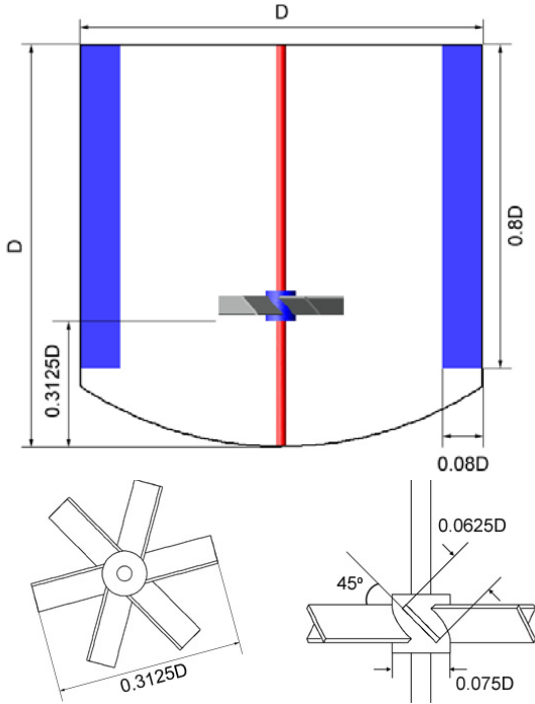
Fig. 1 Agitator geometry
