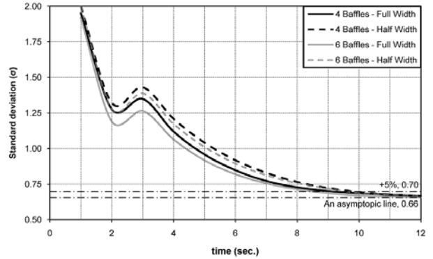
Fig. 7 Influence of baffle design on suspension quality
