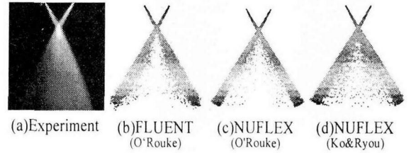
Fig. 6 Validation of spray collision models
