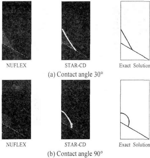
Fig. 2 Comparison of interfacial tracking results between NUFLEX and STAR-CD
