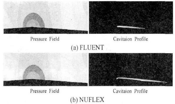
Fig. 3 Comparison of cavitation results between NUFLEX and FLUENT
