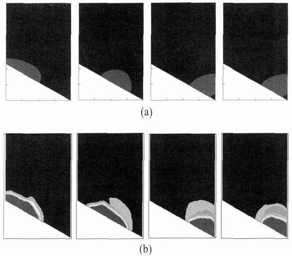
Fig. 3 Comparison of droplet motion obtained from (a) NUFLEX and (b) STAR-CD at \varphi = 90^\circ and Fr=0.2
