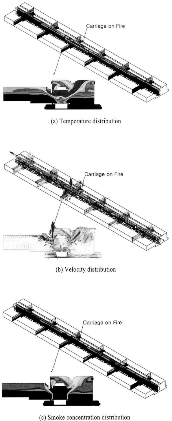
Fig. 5 Computational results at 35sec after fire occurrence for Overplatform Supply / Underplatform Supply ventilation (OSUS)
