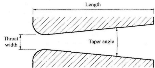
Fig. 3 Geometry of the diffuser/nozzle element.
