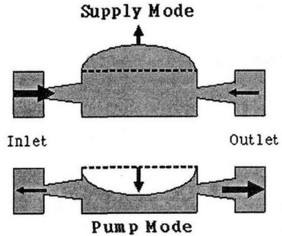
Fig. 1 Operation principle of a micro-pump with two diffuser/nozzle.
