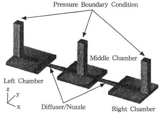
Fig. 2 Computational mesh for the micro-pump.
