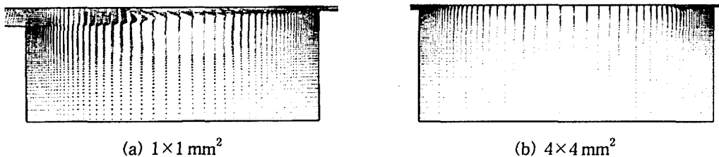
Fig. 11 Velocity profile in the middle chamber (Δp=35 kPa, θ=6.3°).
